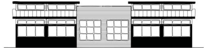
Front Elevation - Plan "B" - With Clerestory
