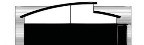
Side Elevation - Plan "B" - With Clerestory
